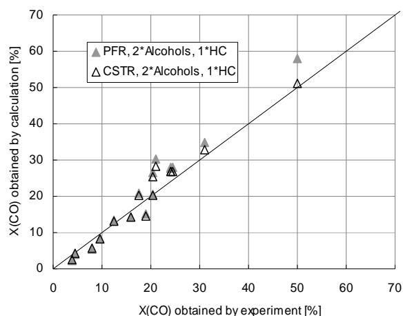
Figure B26. Parity plot for CO conversion - X(\text{CO}) calculated for PFR (solid points) and CSTR (open points) reactor using the gross rates multiplied by the constant factor 2 for alcohols and 1 for HC on the basis of data from [13].
