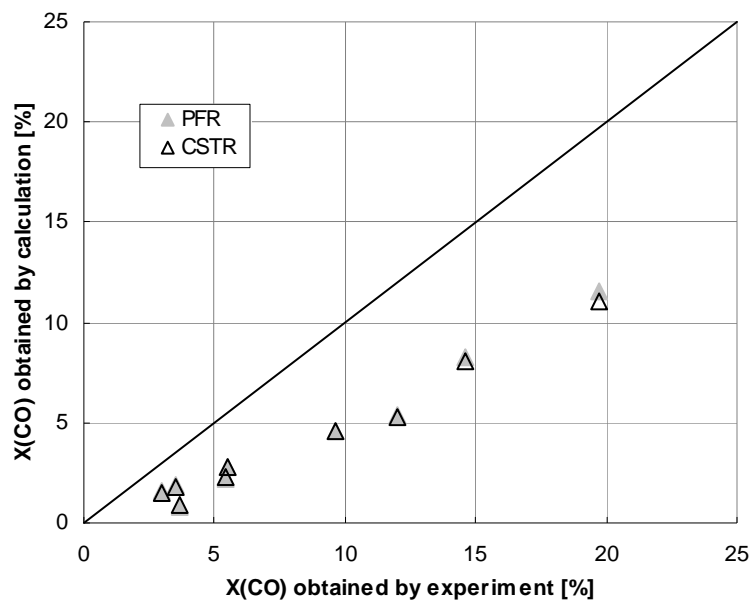
Figure B8. Parity plot for CO conversion - X(\text{CO}) calculated for PFR (solid points) and CSTR (open points) reactor on the basis of data from Li (Gunturu catalyst).
