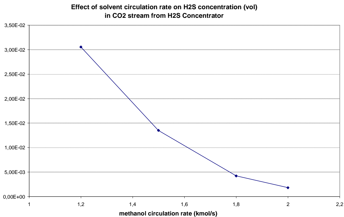
Figure C4: Effect of solvent circulation rate
