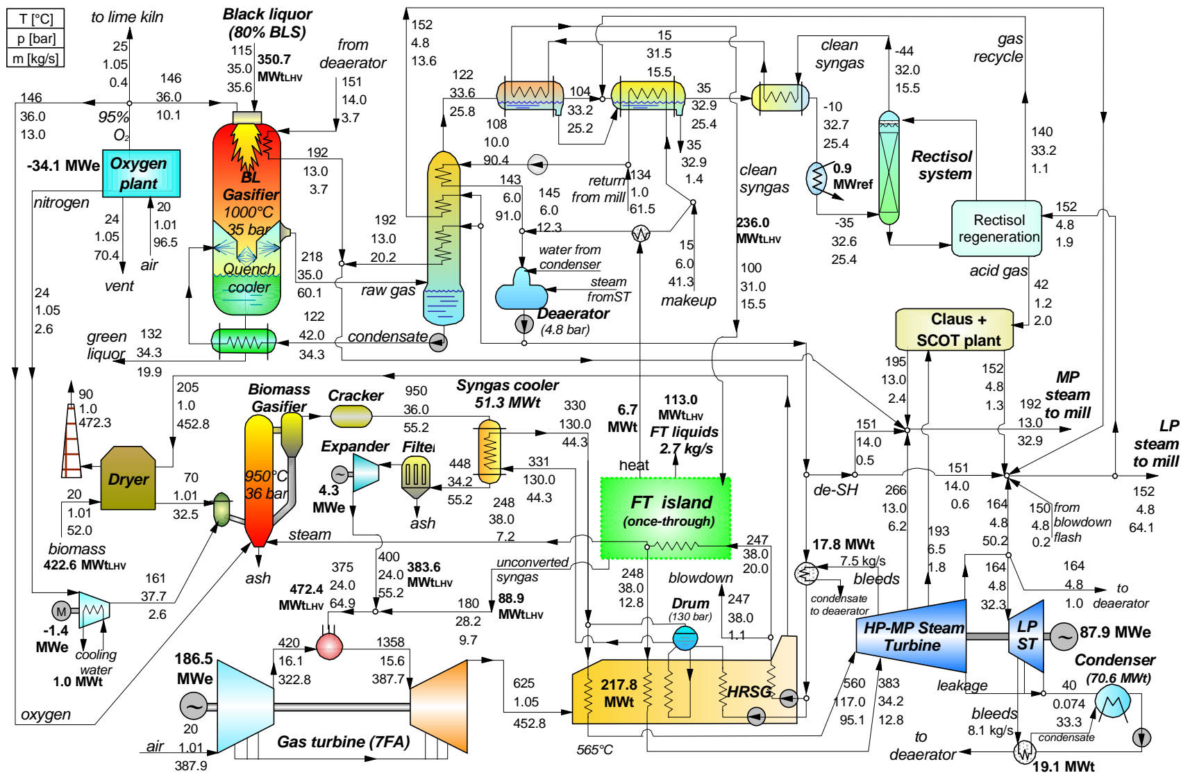
Fig. 22. Plant configuration and mass/energy balances for FTb case
