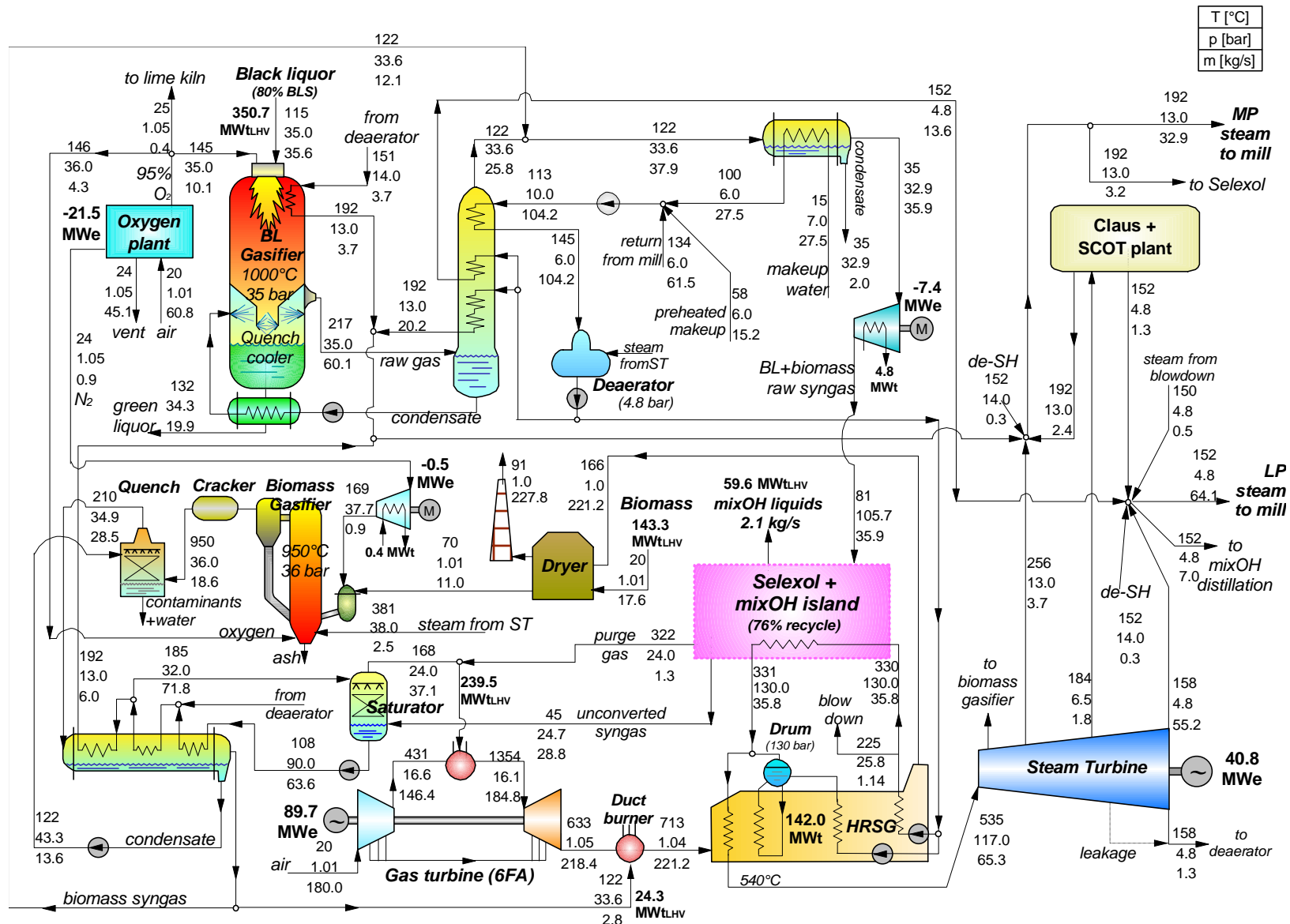
Fig. 24. Plant configuration and mass/energy balances for MixOH case
