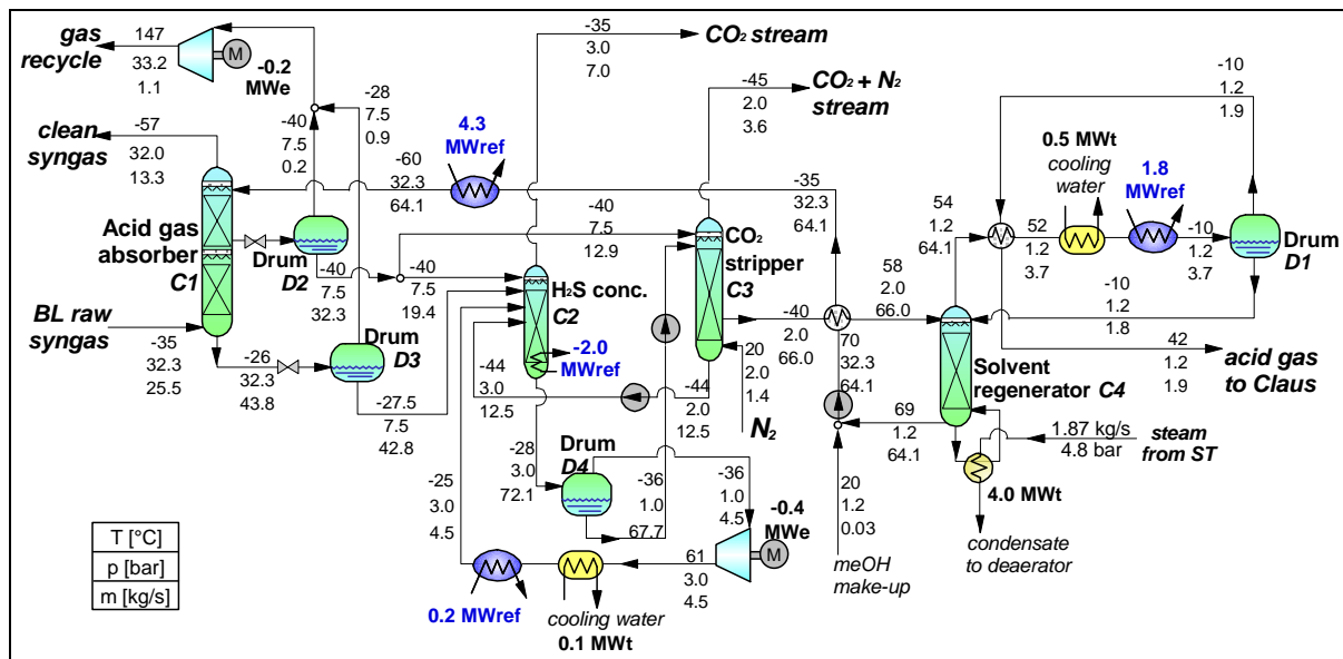
Fig. 9. Energy and mass balances for DMEa and DMEb cases of Rectisol model with \text{H}_2\text{S} and \text{CO}_2 abatement.
