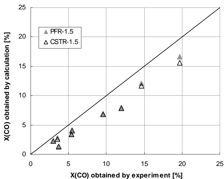
Figure B9. Parity plot for CO conversion - X(\text{CO}) of data from Li for Gunturu catalyst using the gross rates multiplied by the constant factor 1.5.
