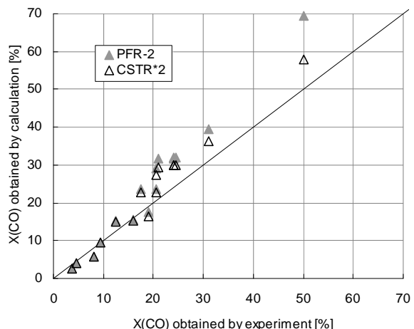
Figure B27. Parity plot for CO conversion - X(\text{CO}) calculated for PFR (solid points) and CSTR (open points) reactor using the gross rates multiplied by the constant factor 2 on the basis of data from [13] (Figure B13).
