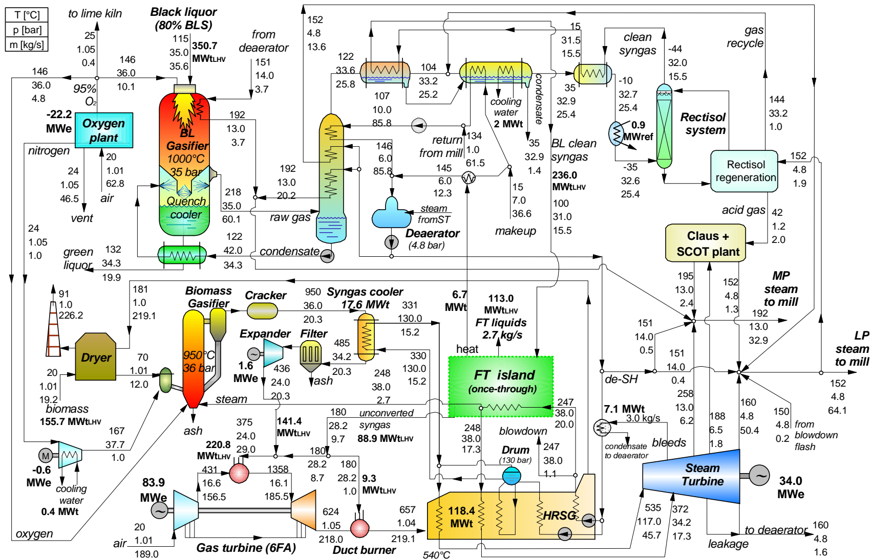
Fig. 21. Plant configuration and mass/energy balances for FTa case
