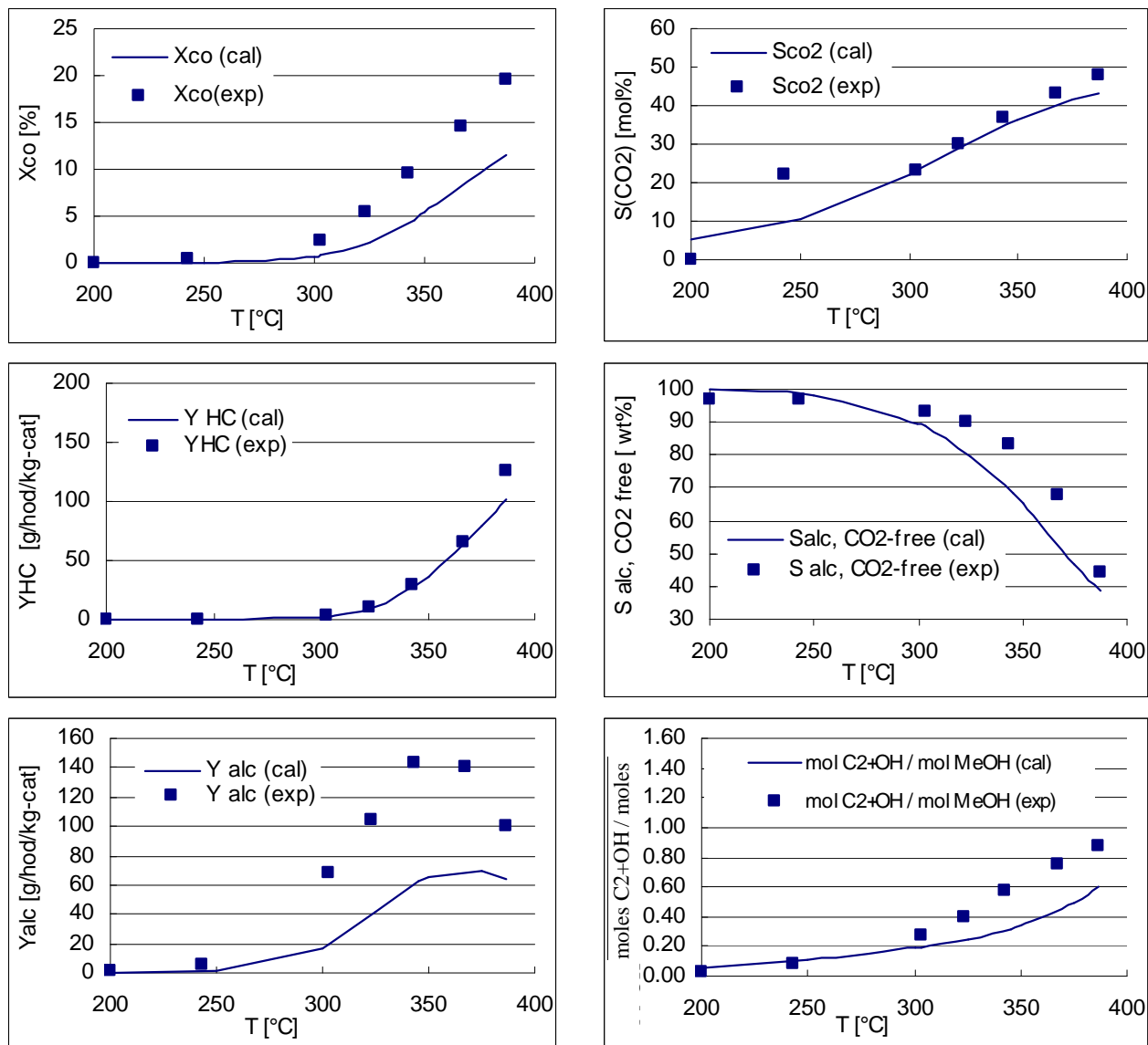
Figure B18. Comparison of experimental [12] and calculated data. Calculated data have been obtained for PF reactor using the gross rates of products without modifications ( 1*PFR ). Experimental conditions: 51 atm, 0.5g cat., H_2=CO=25ml/min (268mol/h/kg-cat.). The following parameters are reported: X_{CO} , conversion of CO; Y_{HC} and Y_{alc} , space-time yields of hydrocarbons and total alcohols (CO 2 -free basis), respectively; and C_2+OH / MeOH , molar ratio of higher alcohols to methanol.
