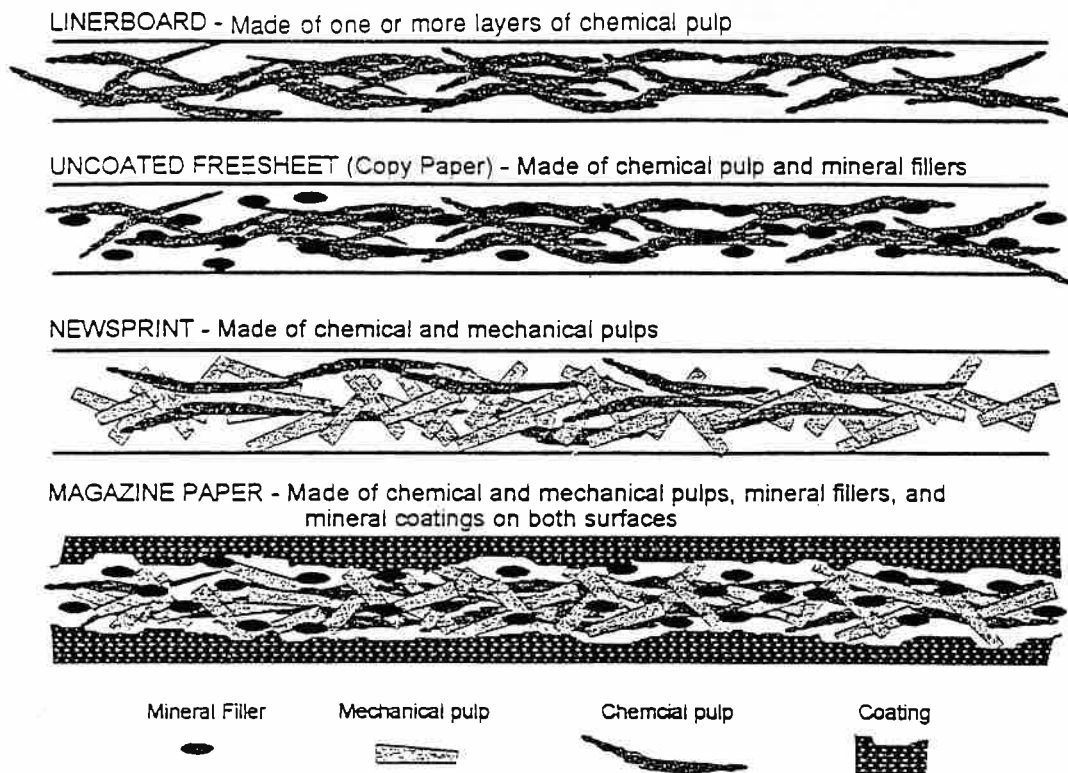
Fig. 2.2. Typical paper and paperboard compositions. Source: R.E. Butner, Simons Eastern, Atlanta, Georgia.
