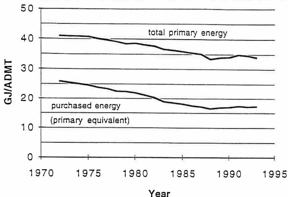
Figure ES1. Total annual primary energy use in the pulp, paper, and paperboard industry between 1972 and 1993 in Gigajoules per air-dry metric tonne of production (one GJ/ADMT is 0.86 MBtu/air-dried short tonne).
